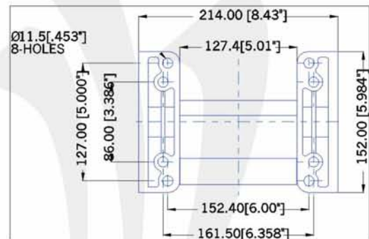
Bottom View (Mount Pattern)
